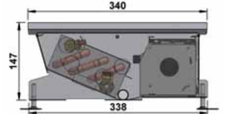
COIL – HCM
