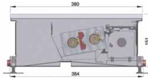
COIL – KO2
