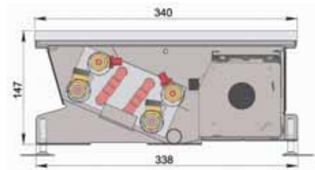
COIL – HCM4pipe
